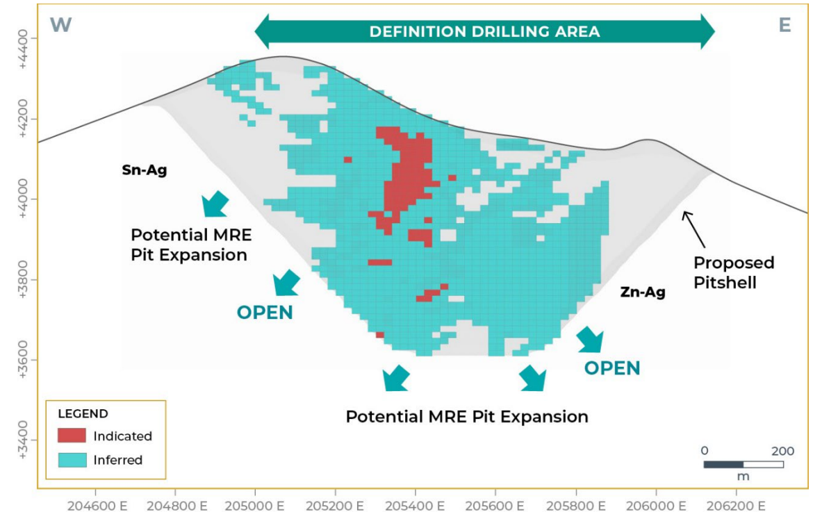
Optimized Pit Showing Mineral Resource Classification
